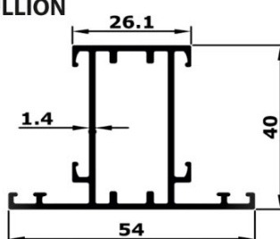
MULLION
