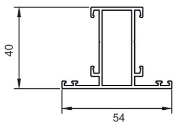
MULLION
