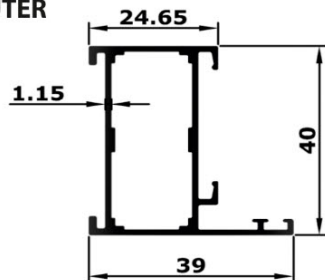
OUTER
