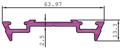
PRESSURE PLATE
